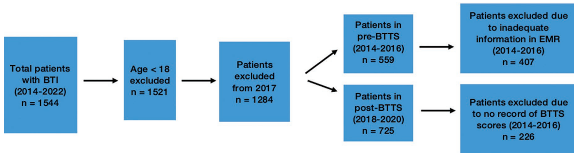
Figure 1. Flowchart.
